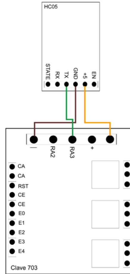
RECEPTOR BT-RR3
